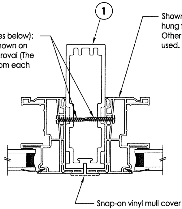
1 HORIZONTAL CROSS SECTION 2 6580 Mullion to Window Connection
